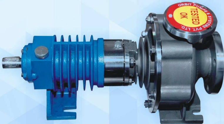
HORIZONTAL CENTRIFUGAL METALLIC JACKETED PROCESS PUMPS, (MOC : C. I., C. S., SS-304 / 316, ALLOY-20, H-B, H-C ETC)
